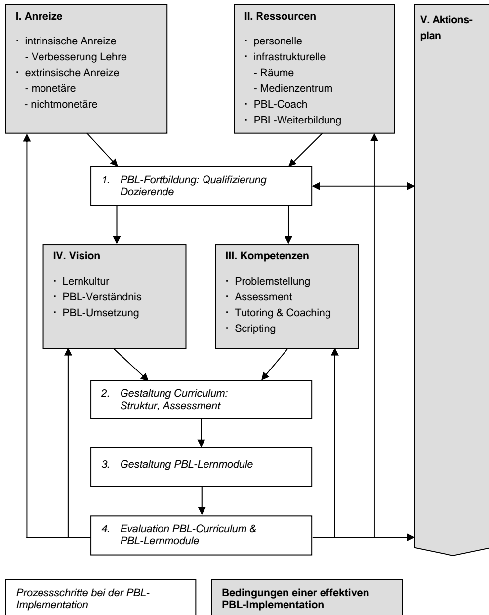
Abb. 3: PBL-Implementationsmodell
